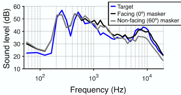
Fig. 1. Long-term magnitude spectrum for the target, facing ( 0^\circ ) masker, and the nonfacing ( 60^\circ ) masker. Color reflects stimulus type, as defined in the legend.
